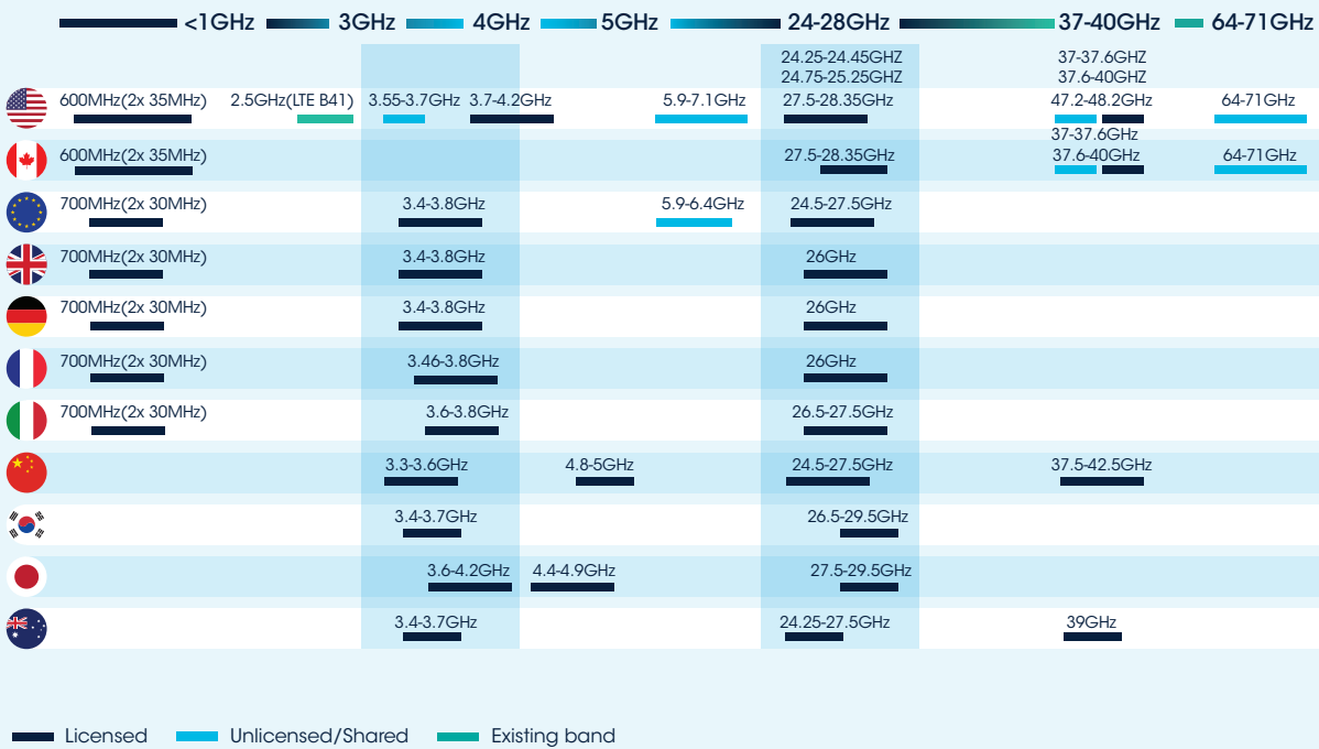
FIGURE 12: GLOBAL SNAPSHOT OF 5G SPECTRUM
